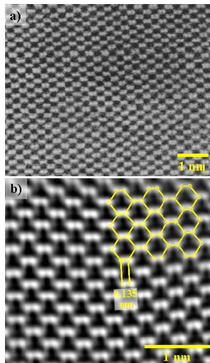
Figure 2 STEM images of Si dumbbells in 110-oriented silicon. (a) is a raw image showing the dumbbells. (b) is a low-pass filtered, expanded image with atomic positions labeled.
